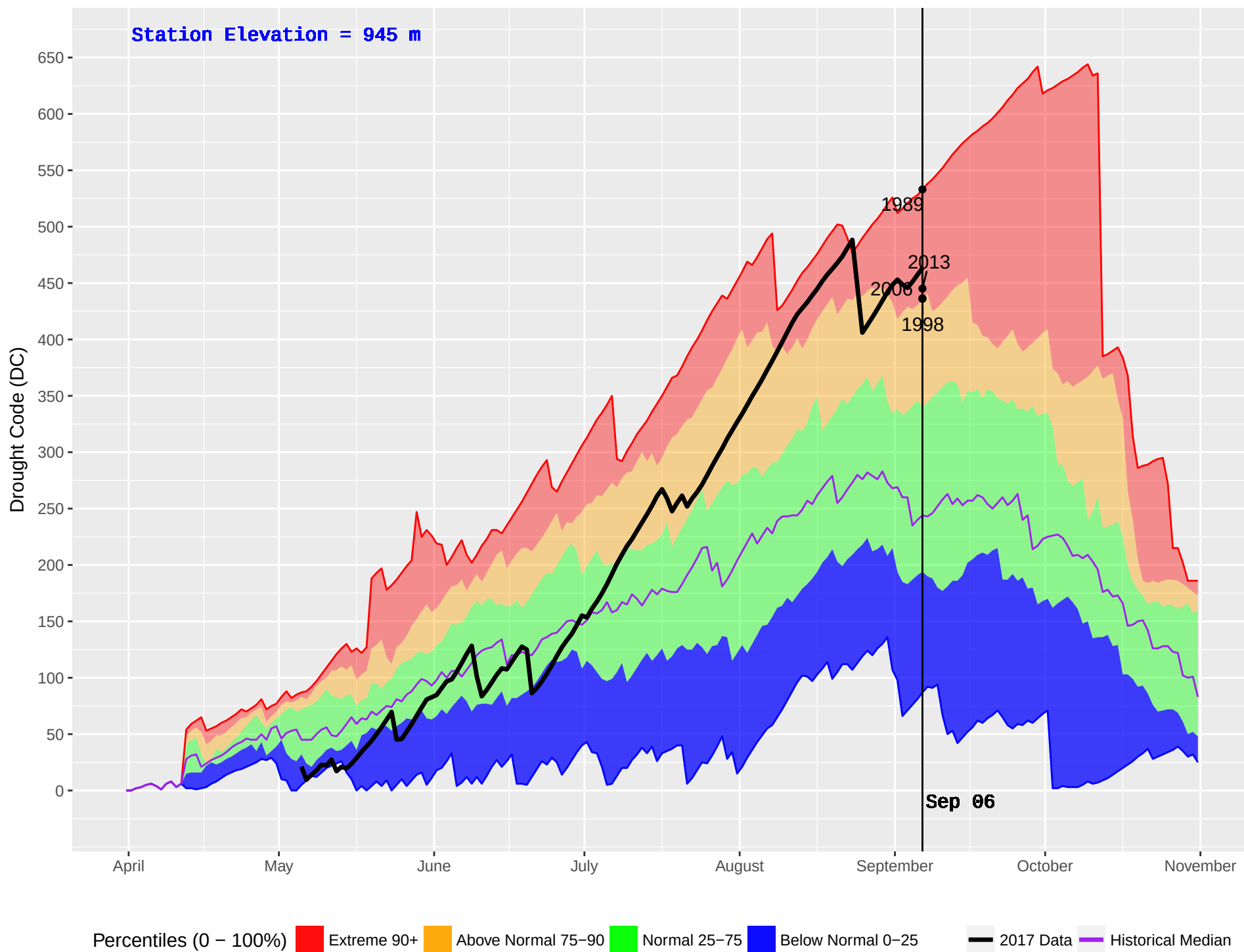
BOWRON HAGGEN (193) : Historical (1986–2016) and Current (2017) Noon Drought Code (DC)
