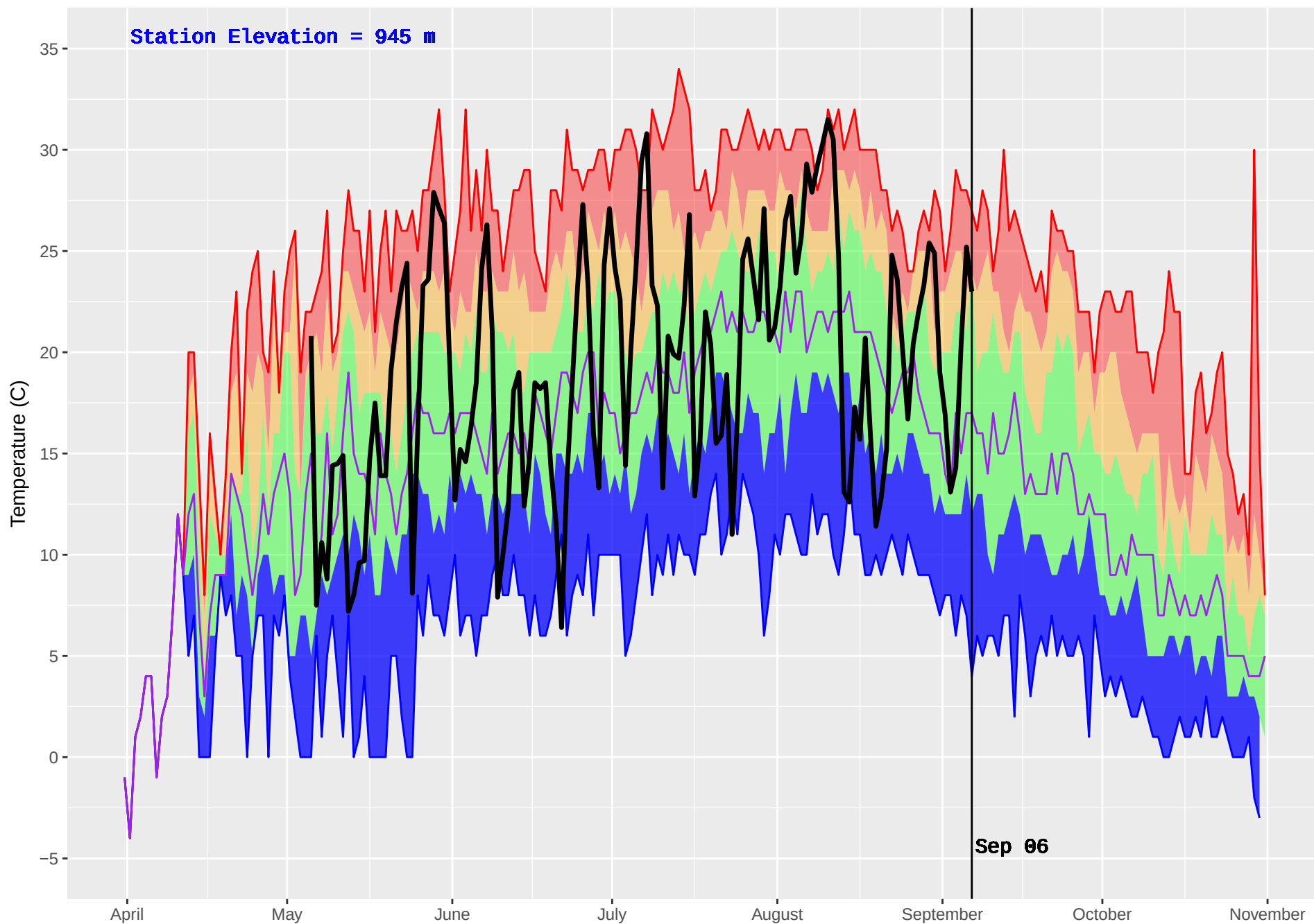
BOWRON HAGGEN (193) : Historical (1986–2016) and Current (2017) Noon Temperature
